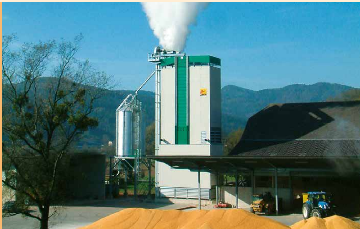
■ Industrial dryer ERCL with slow cooling system.
